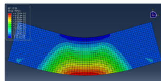
Finite Element (FE) Model of Flexural Test
