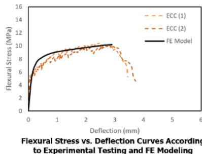
Figure 3. Finite element modeling of ECC under flexural loading.
