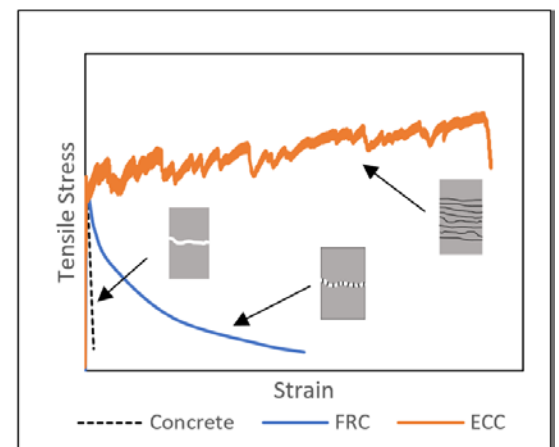
Figure 1. Stress versus strain behavior of cementitious materials in tension.
